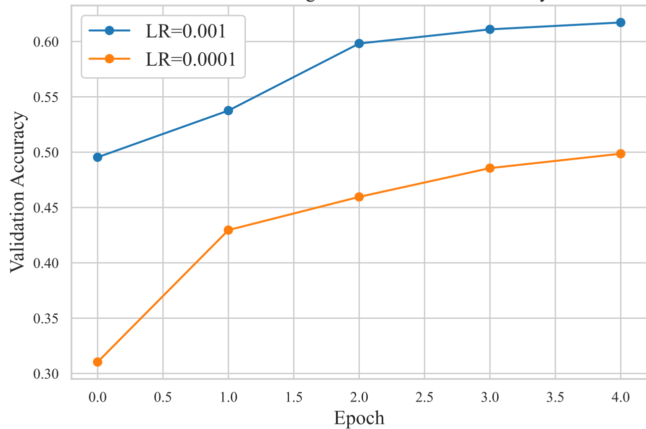
Effect of Learning Rate on Validation Accuracy
